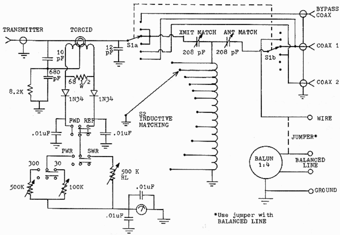
MFJ-941D SCHEMATIC DIAGRAM
